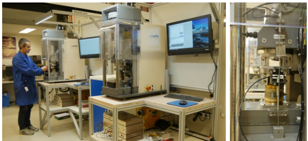
Fig.1 GDS' Electromechanical Direct Simple Shear apparatus in NGI laboratory in Oslo.
