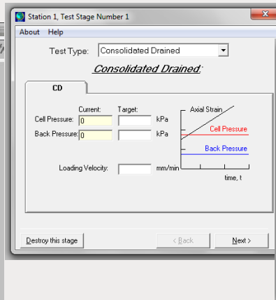
Fig. 2 Show a typical test stage in GDSLAB
