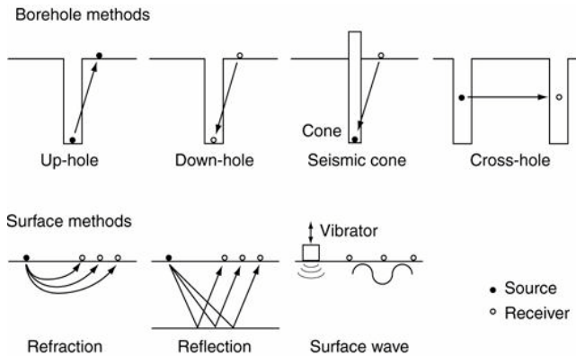
Fig. 10. Seismic Methods
